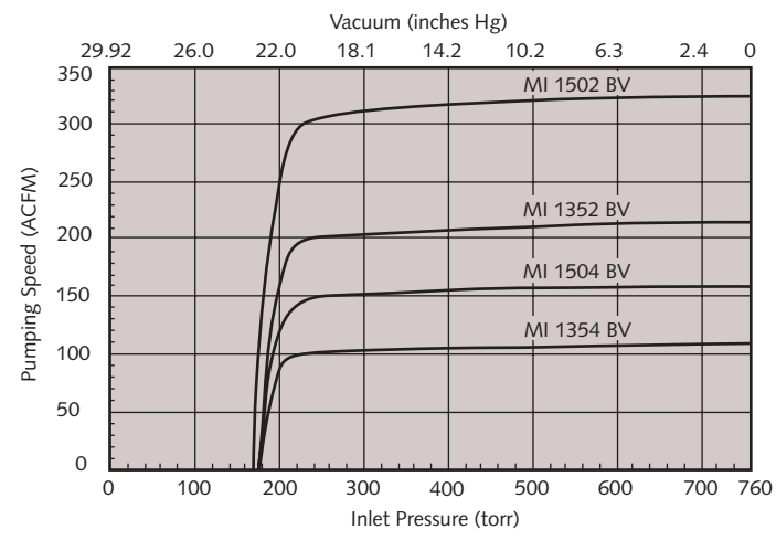
Pumping Speed vs. Inlet Pressure
