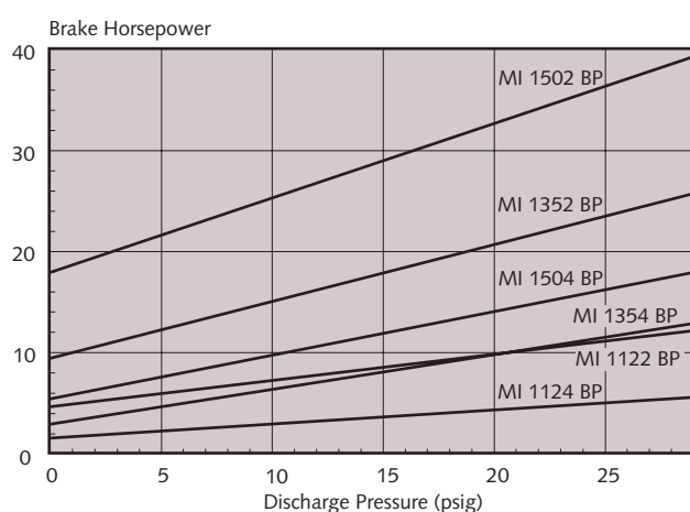
Brake Horsepower vs. Discharge Pressure
