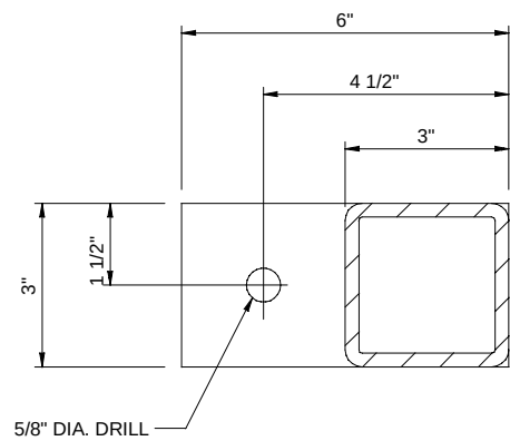
SECTION A-A FOOT PAD DETAIL SCALE: HALF SIZE TYPICAL - 12 PLACES
