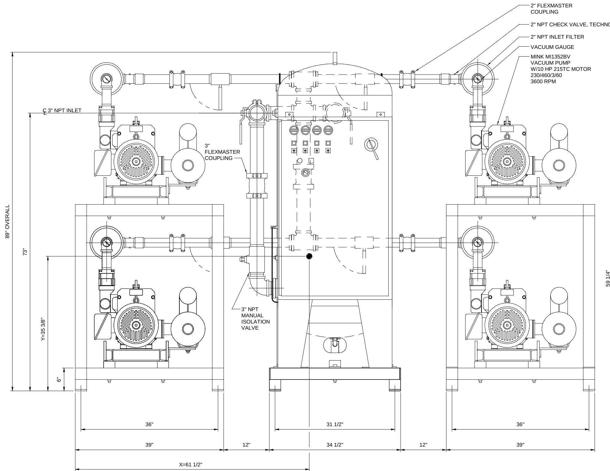
FRONT ELEVATION
