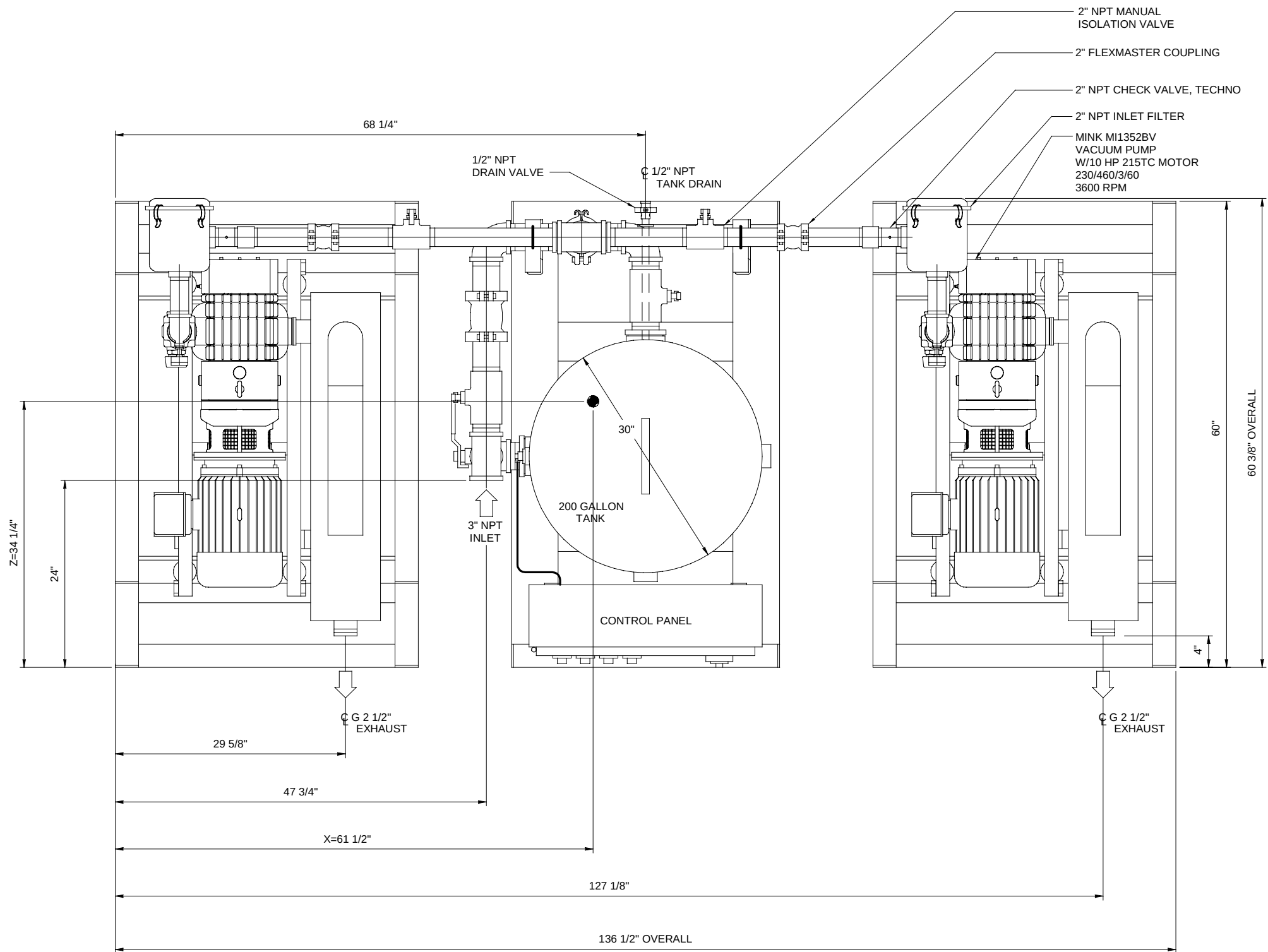
PLAN VIEW
