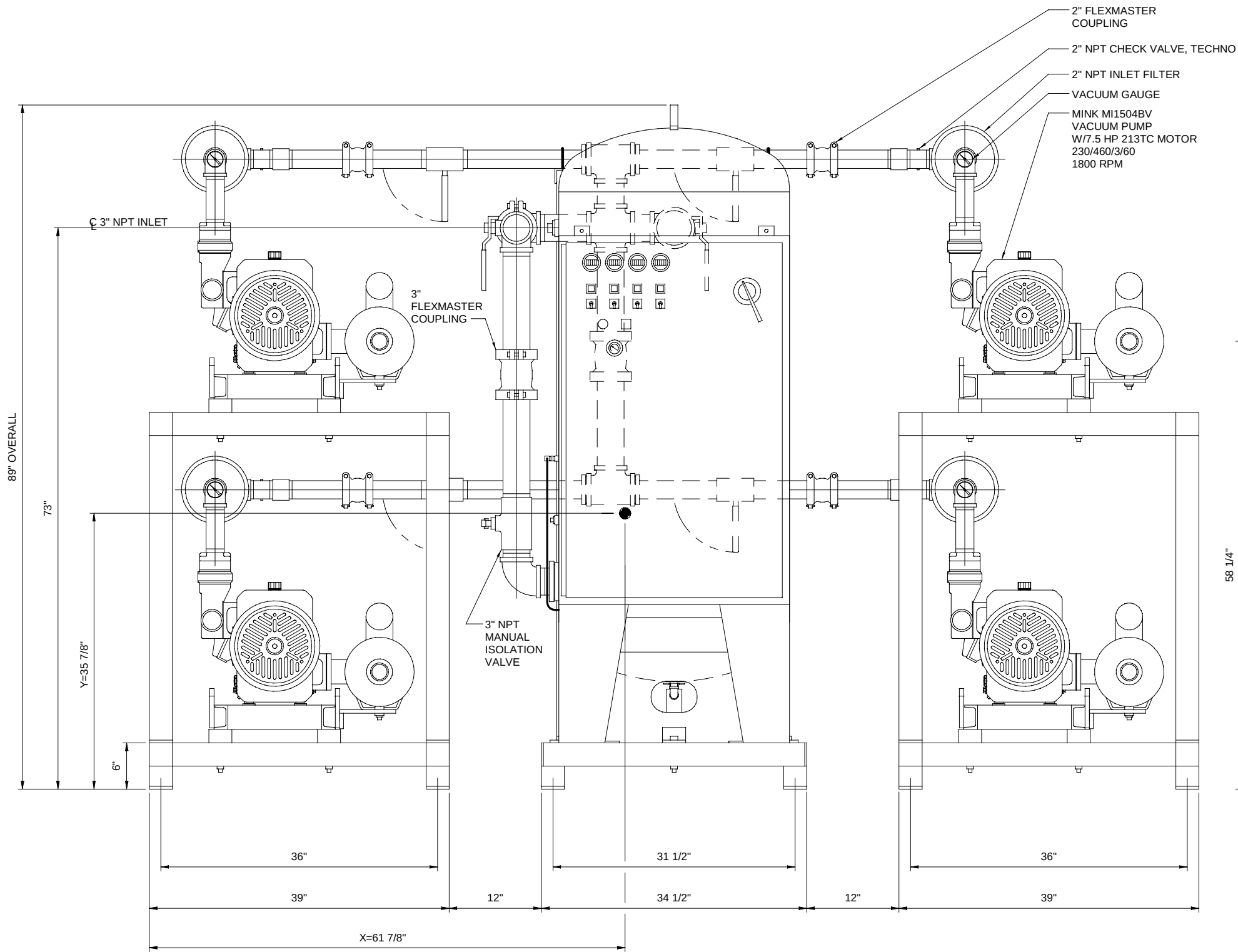
FRONT ELEVATION
