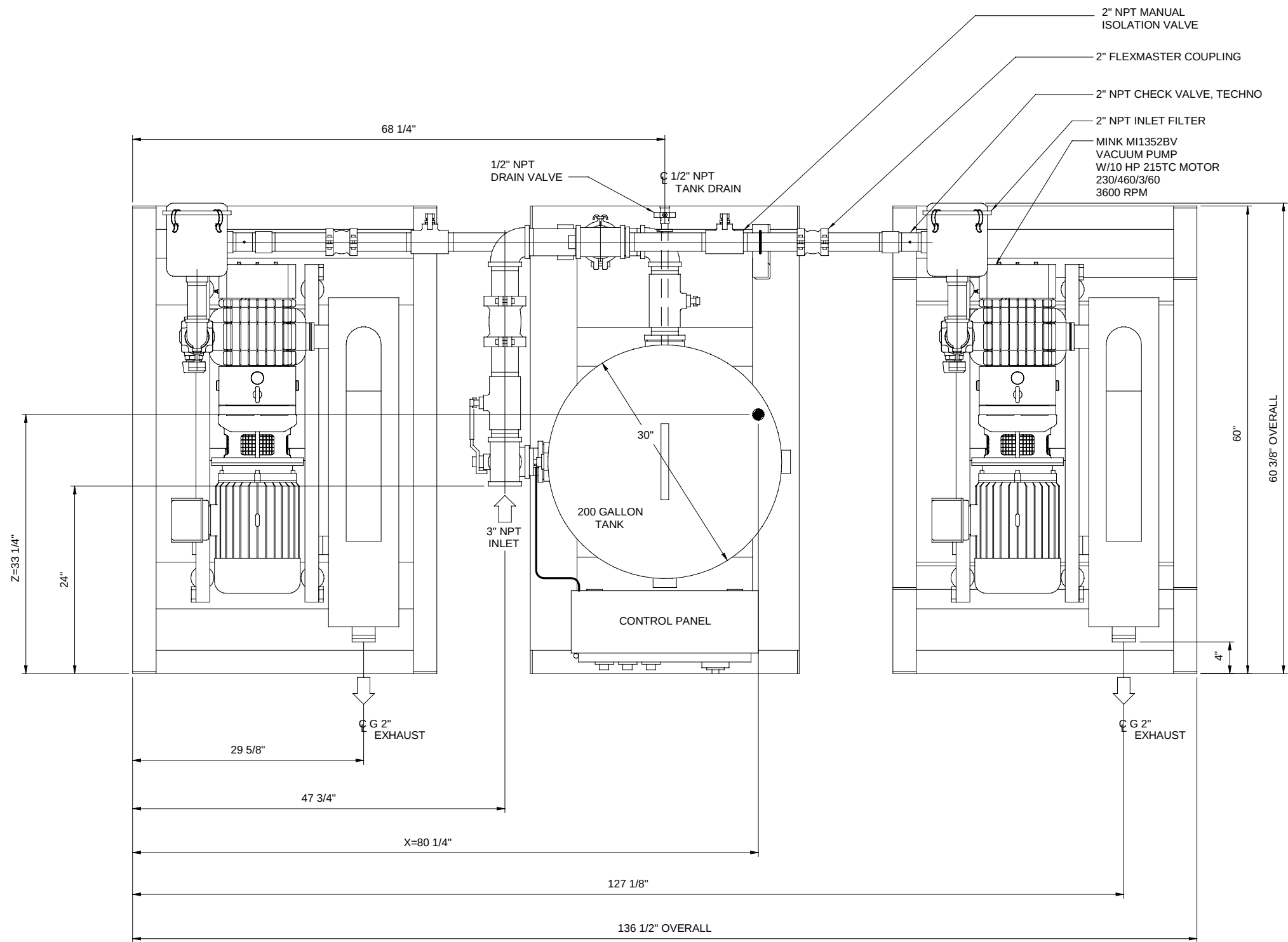
PLAN VIEW
