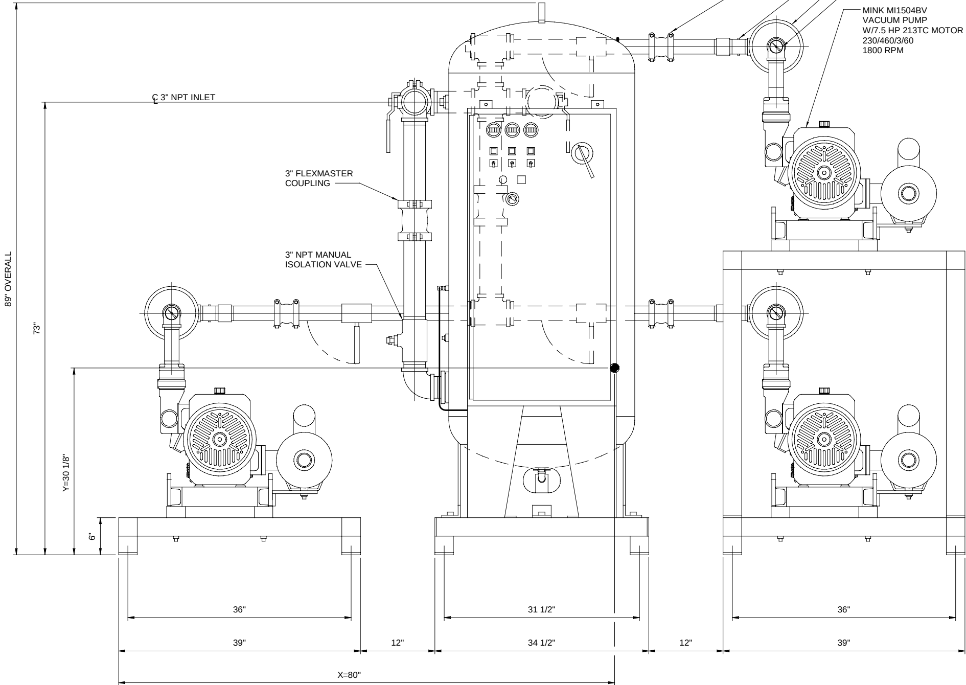
FRONT ELEVATION
