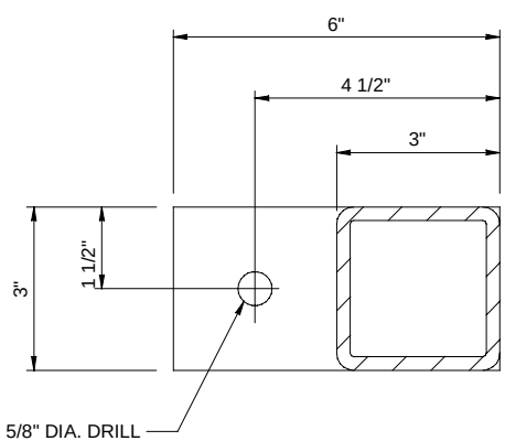
SECTION A-A FOOT PAD DETAIL SCALE: HALF SIZE TYPICAL - 8 PLACES
