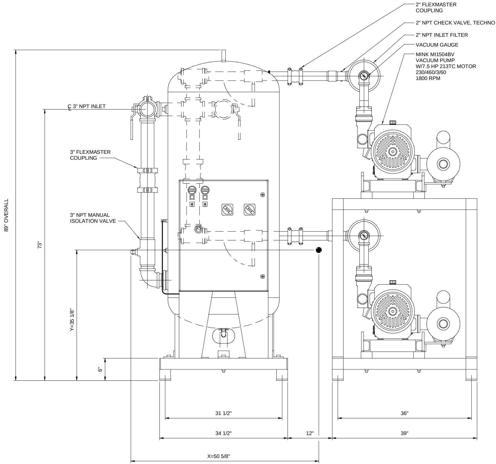
FRONT ELEVATION
