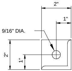
SECTION A-A FOOT PAD DETAIL TYPICAL - 4 PLACES SCALE - 1/2" = 1"
