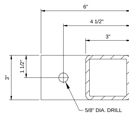
SECTION A-A FOOT PAD DETAIL SCALE: HALF SIZE TYPICAL - 20 PLACES
