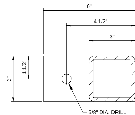
SECTION A-A FOOT PAD DETAIL SCALE: HALF SIZE TYPICAL - 20 PLACES
