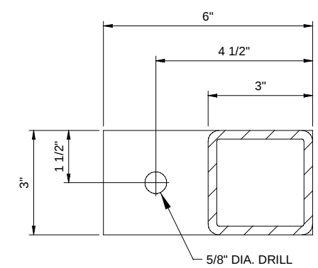
SECTION A-A FOOT PAD DETAIL SCALE: HALF SIZE TYPICAL - 16 PLACES
