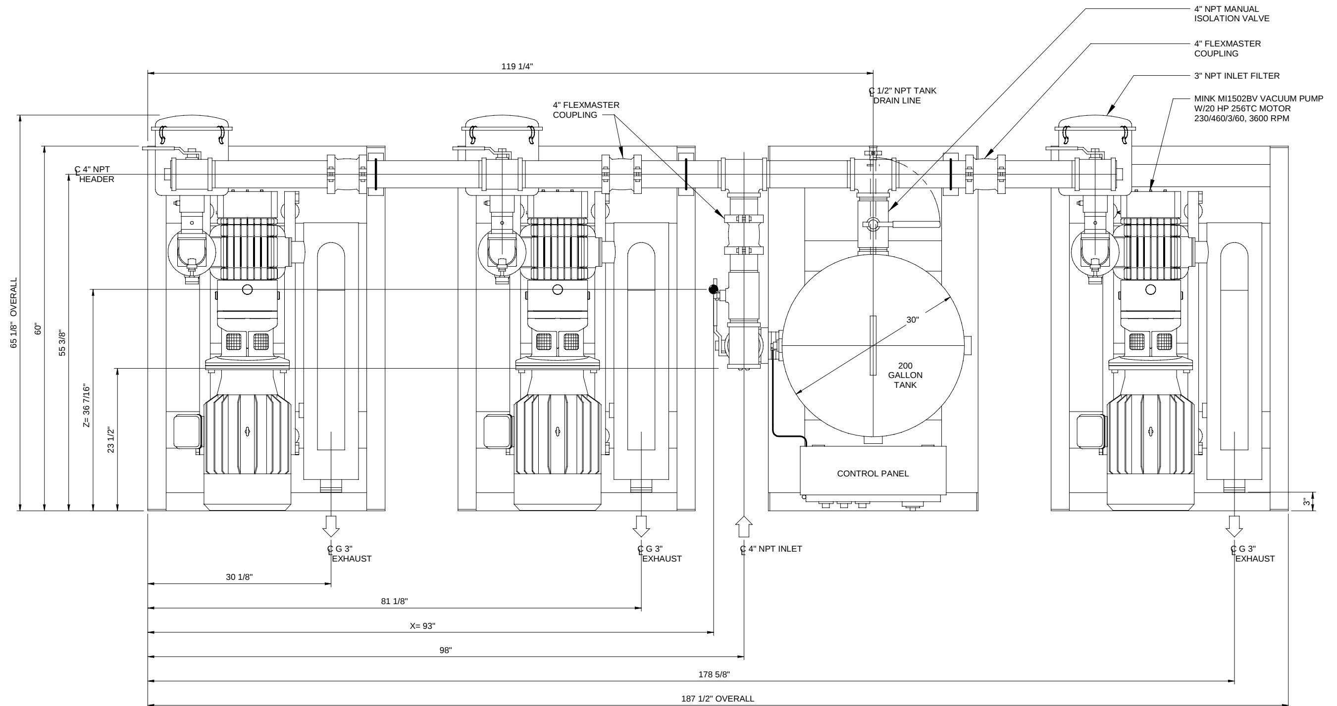
PLAN VIEW
