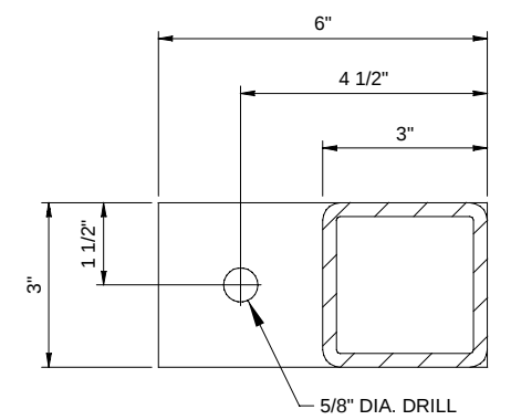
SECTION A-A FOOT PAD DETAIL SCALE: HALF SIZE TYPICAL - 12 PLACES
