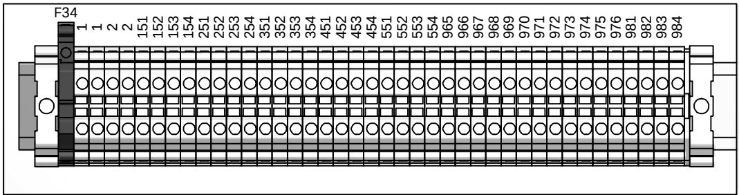
DETAIL A
