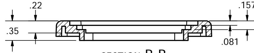
SECTION B-B
